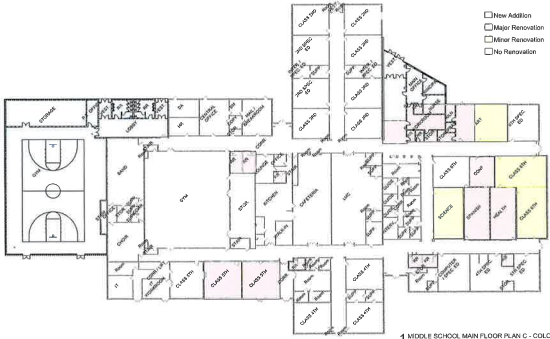
1 MIDDLE SCHOOL MAIN FLOOR PLAN C - COLOR CODED SCALE: 1" = 30'
